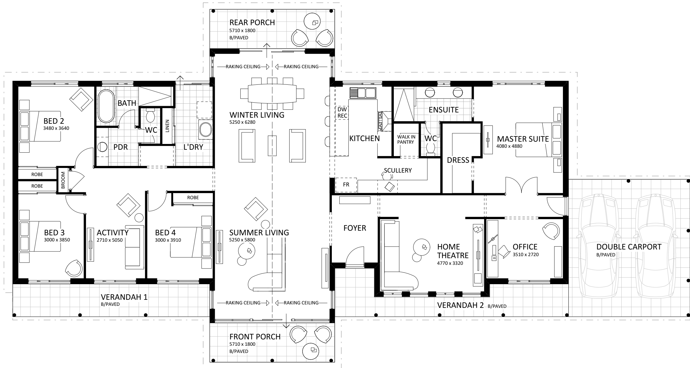
FLOOR PLAN 1:100
